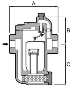
No. 980 SERIES DIMENSIONS (MM). MOP(KG/CM 2 ). WT(KG)
