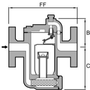
No. 991 SERIES
